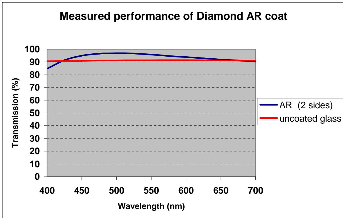
Fig 1 Typical Chart showing standard AR (anti reflective) coating produced at Diamond Coatings on 2mm glass
